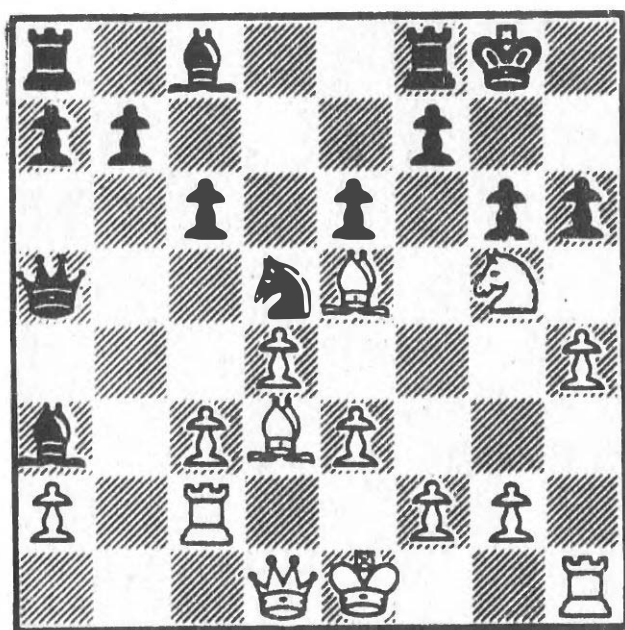
499 After 16...g6
